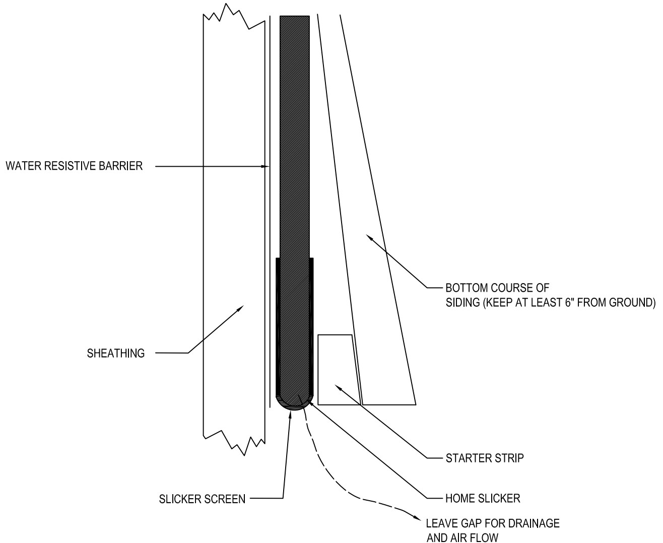
BOTTOM DETAIL
